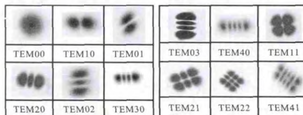
(a) 激光横模 (a) Laser transverse mode
