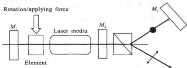
图 2 激光器本身作为传感器 Fig.2 Laser working as a sensor
